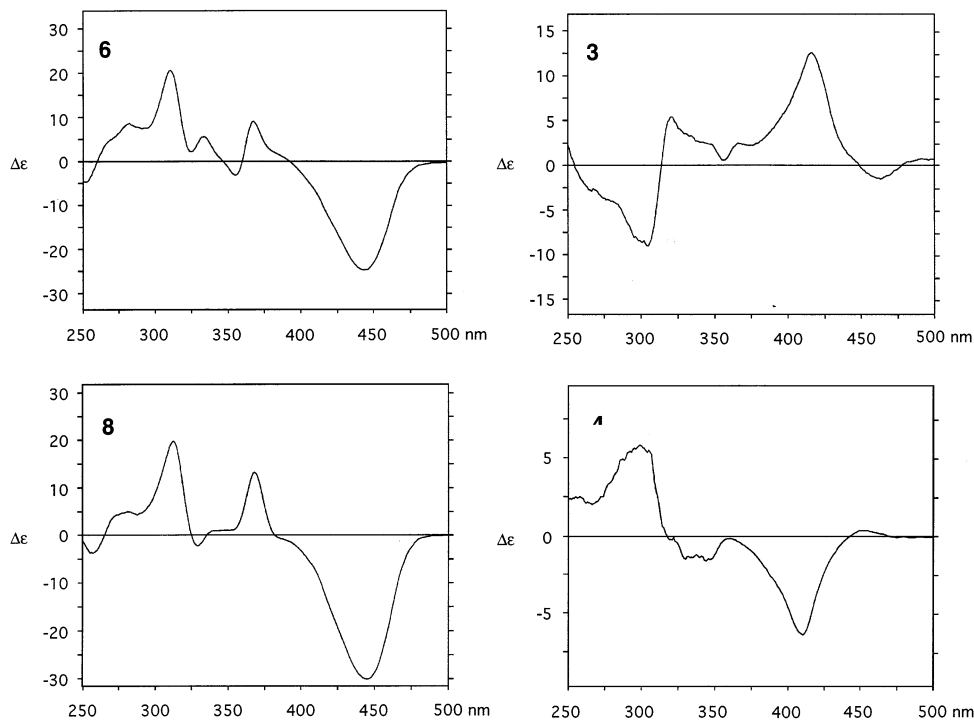
Fig. 11. CD-spectra of \Delta -Pt(th4,5ppy) 2 (3), \Delta -Pt(th4,5capy) 2 (4), \Delta -Pt(th5,6ppy) 2 (6) and \Delta -Pt(th5,6capy) 2 (8) [196].
