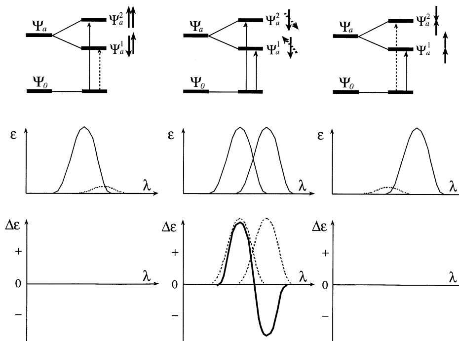
Fig. 5. Exciton coupling of two degenerate transitions.
