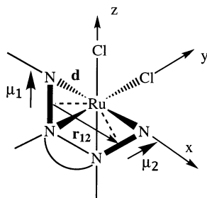
Scheme 4.
