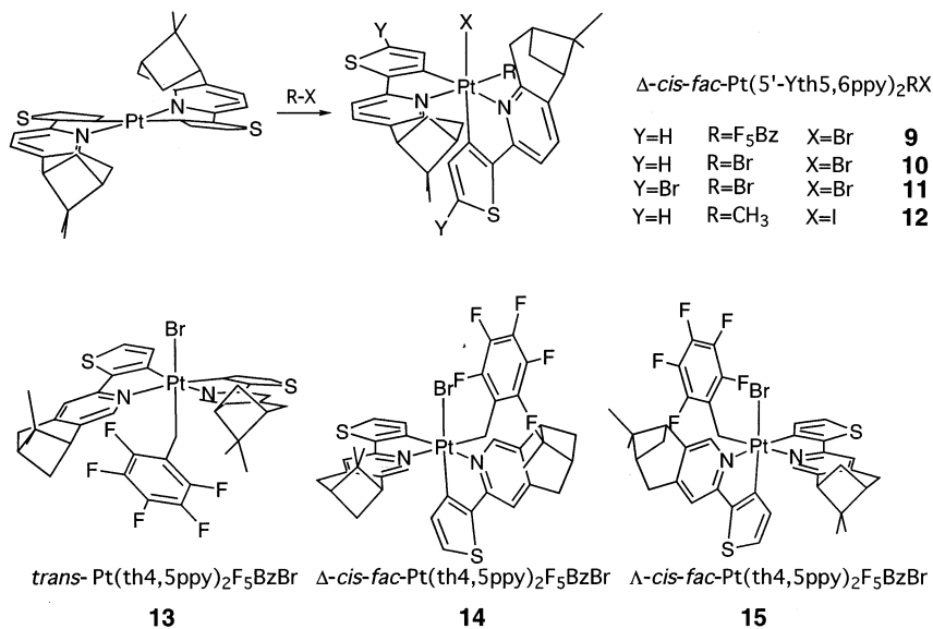
Scheme 9.
