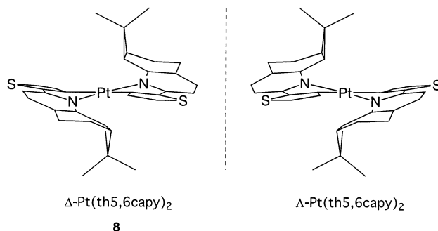
Fig. 9. Enantiomers of Pt(th5,6capy) 2 derived from (+)-2-carene and (–)-2-carene.
